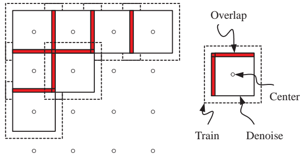
Fig. 1. Description of the denoising process. Denoising is done for each patch, labeled “Denoise” using the PC denoising algorithm. Training set for determining the principal components is generated from the patch labeled “Train”. The “Denoise” patches are overlapped in the dark region labeled “Overlap” in order to eliminate blocking artifacts.
